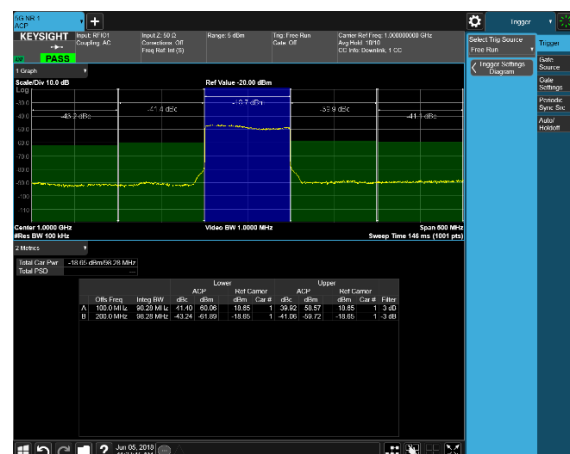
Figure 2. 5G NR adjacent channel power (ACP) results
