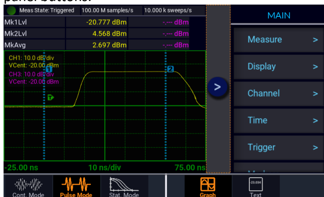
Figure 4-1. Pulse Mode Main Menu
