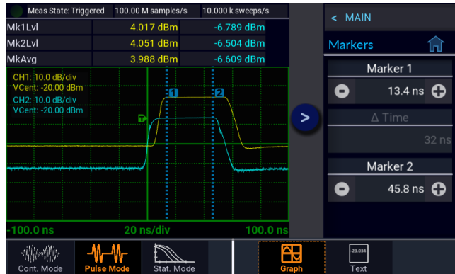
Figure 3-6. Marker Measurements on CH1 and CH2 Pulses
